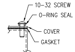
COVER AND SCREW DETAIL
