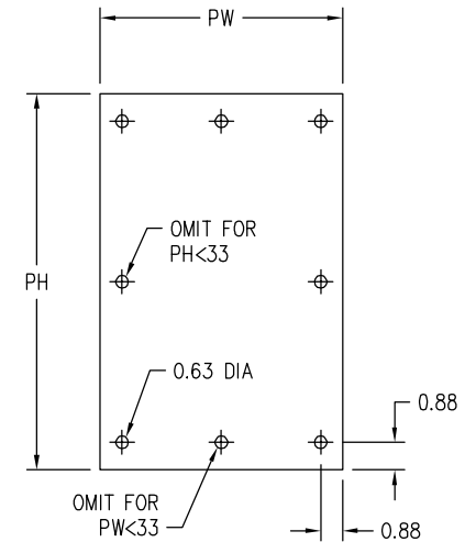
BACK PANEL DIMENSIONS
